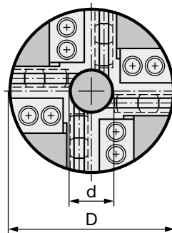
Tool head with HSK-holder, form A automatic
